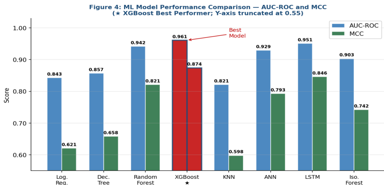
Figure 4: ML Model Performance Comparison — AUC-ROC and MCC by Classifier (Y-axis truncated at 0.55). XGBoost (★) leads across both metrics. LSTM competitive on temporal fraud pattern detection. Red bars = XGBoost. Source: Authors' analysis.
