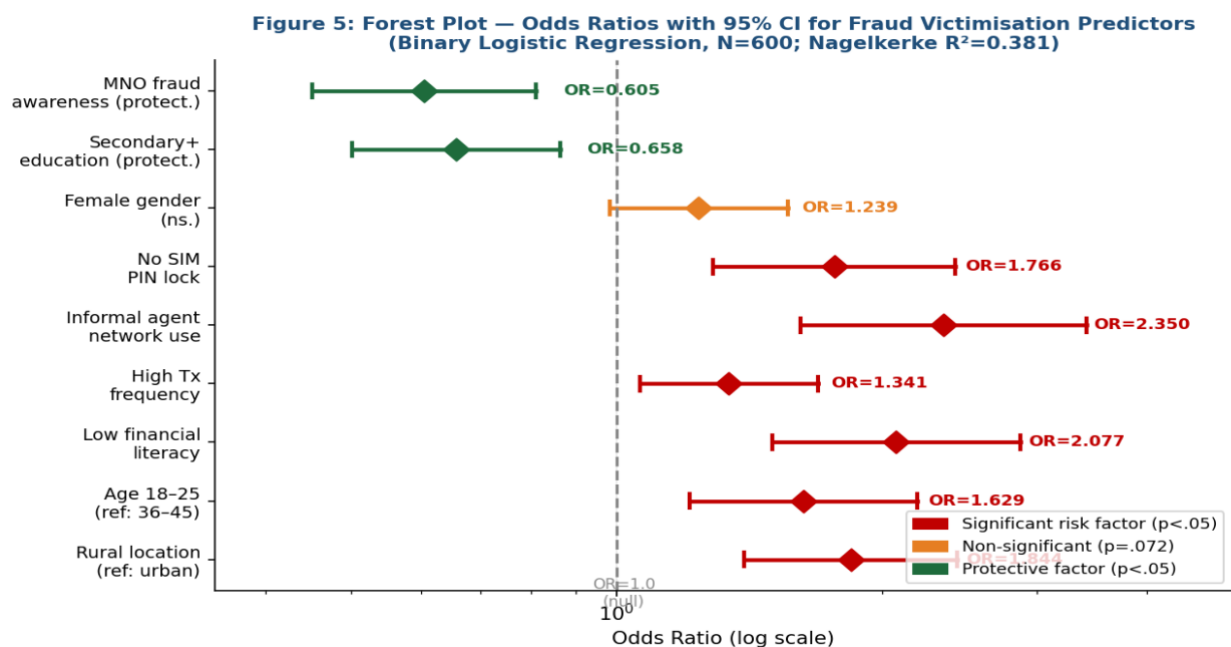
Figure 5: Forest Plot—Odds Ratios with 95% CI for Fraud Victimization Predictors (Logistic Regression, N=600; Nagelkerke R^2=0.381 ). Diamond = OR point estimate; horizontal bars = 95% CI. Red = significant risk factors; orange = non-significant; green = protective factors. Log-scale x-axis. Source: Authors' analysis.
