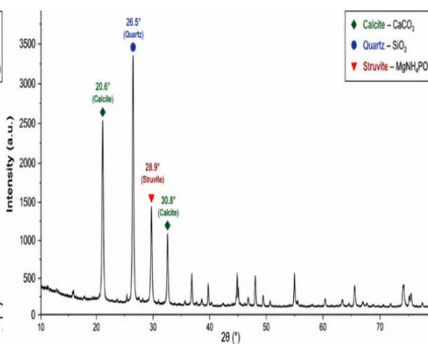
Figure 3.2: XRD of Substrate Pig Manure
