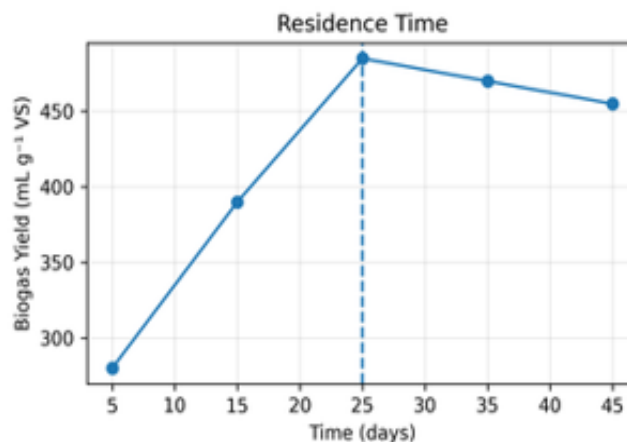
Figure 4.2: OFAT value for Residence Time
