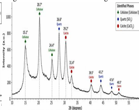
Figure 3.4: XRD of mixed Feedstock (1:1:1)
