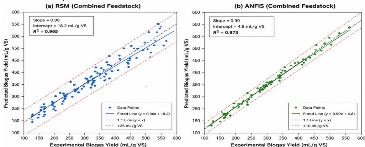
Figure 9 : The scatter plots of predicted vs. experimental biogas yields.
