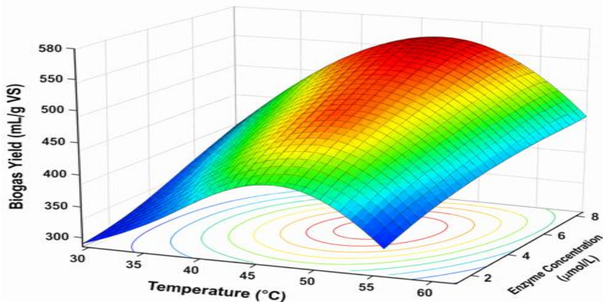
Figure 5.1: Temperature vs. Enzyme Concentration (at fixed time = 25 days, pH = 7)
