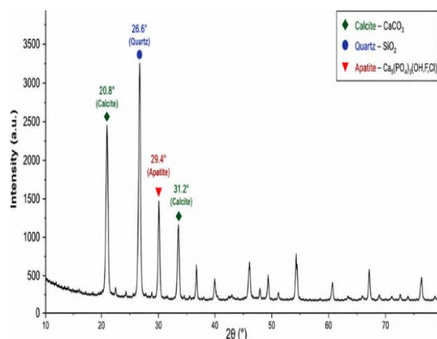
Figure 3.1: XRD of Substrate Poultry Dropping
