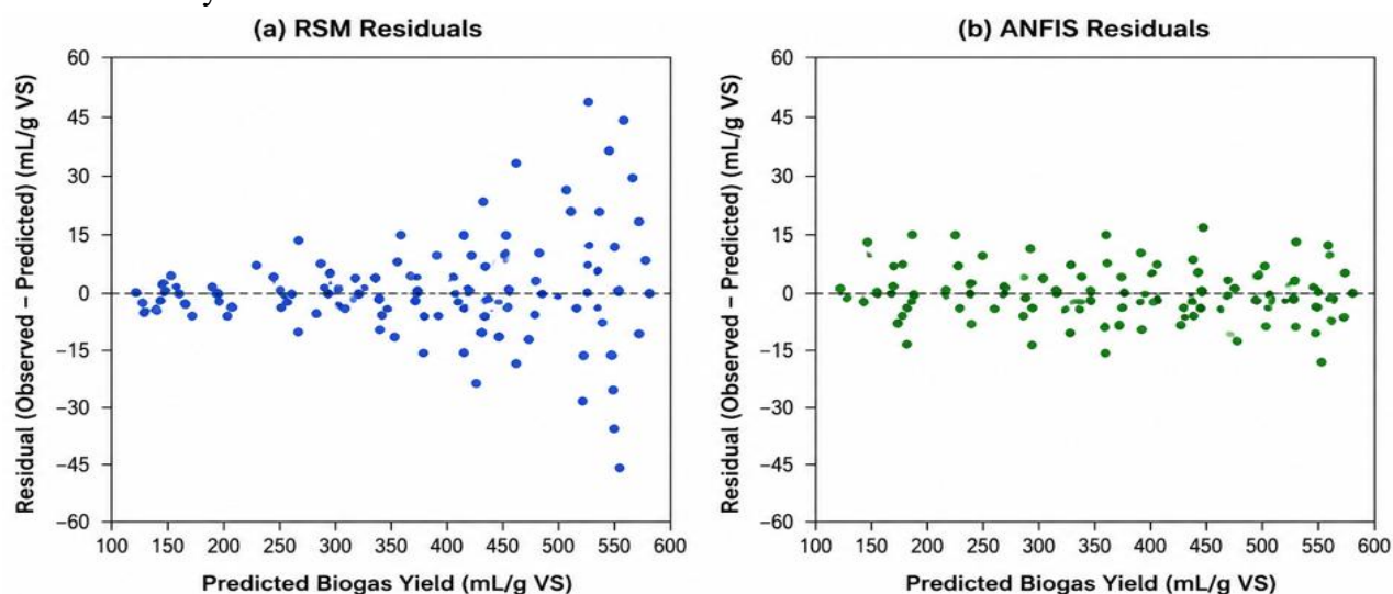
Figure 8: The residual plots for both models.
