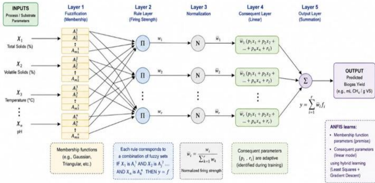
Figure 2: ANFIS Architecture for Biogas Yield Prediction
