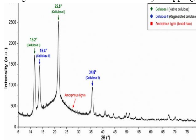
Figure 3.3: XRD of Brewery Spent Grain
