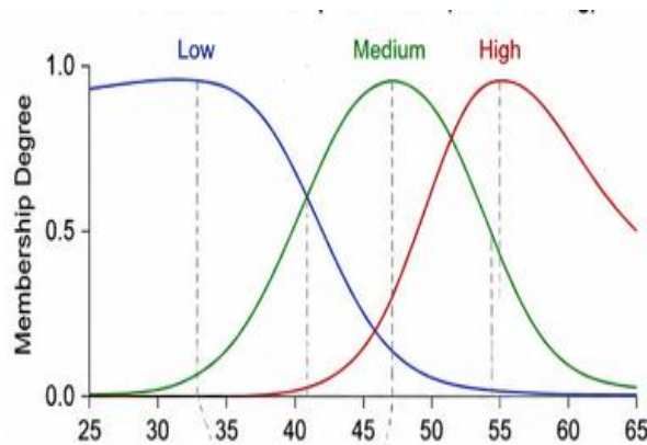
Figure 6.1: ANFIS MF after Training (Temp °C)
