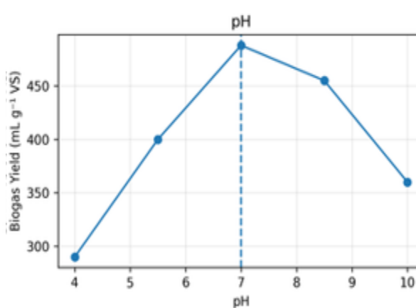
Figure 4.4: Feasibl OFAT value for Ph
