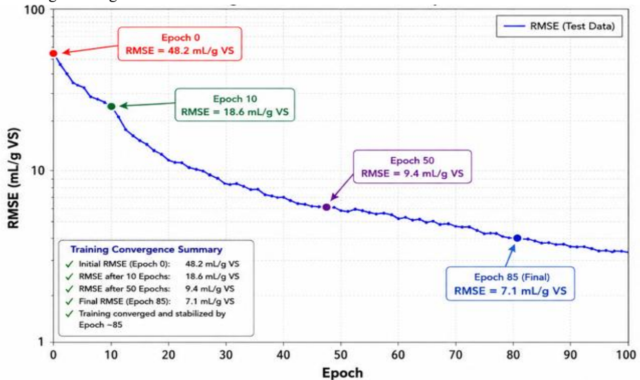
Figure 7: The training error reduction over 100 epochs.
