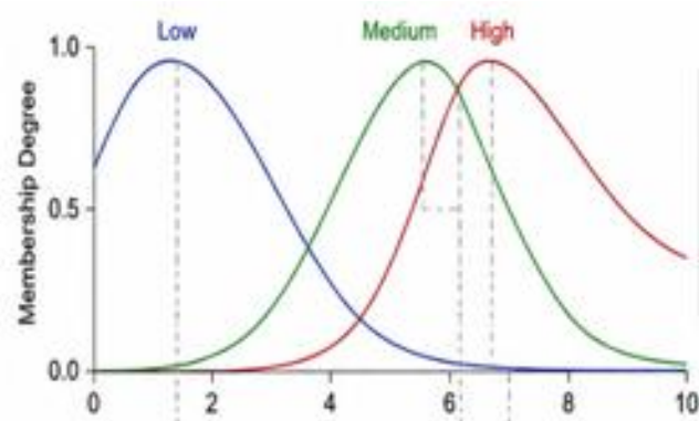
Figure 6.2: ANFIS MF after Training (Enzyme Conc. µmol/L)
