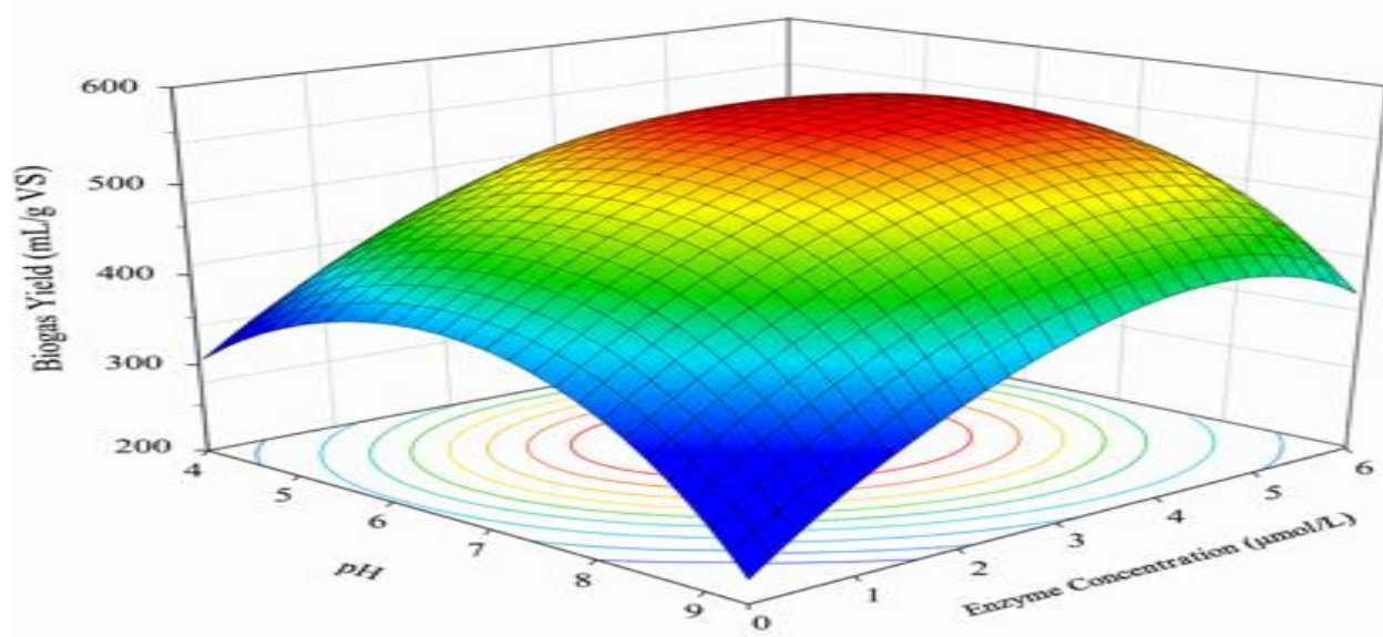
Figure 5.3: pH vs. Enzyme Concentration (at fixed temp = 45°C, time = 25 days)
