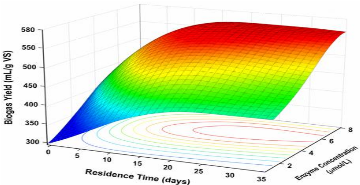
Figure 5.2: Residence Time vs. Enzyme Concentration (at fixed temp = 45°C, pH = 7)
