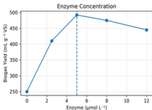
Figure 4.3: OFAT value for Enzyme Conc.
