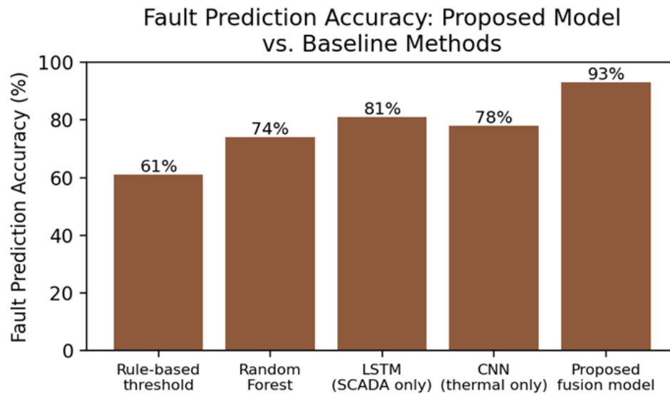
Figure 2: Fault Prediction Accuracy Proposed Model vs. Baseline Methods
