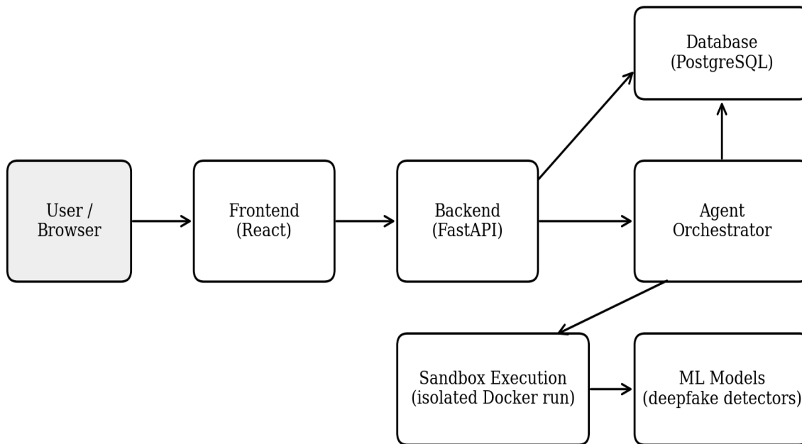
Fig. 1. System architecture of the AI-powered deepfake detection tool.
