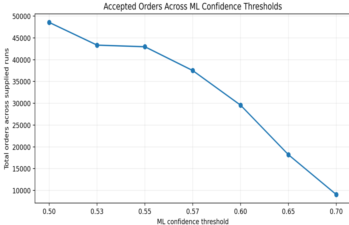
Figure 2. Total recorded orders across the supplied ML-assisted experiment runs as the validation threshold increases.
