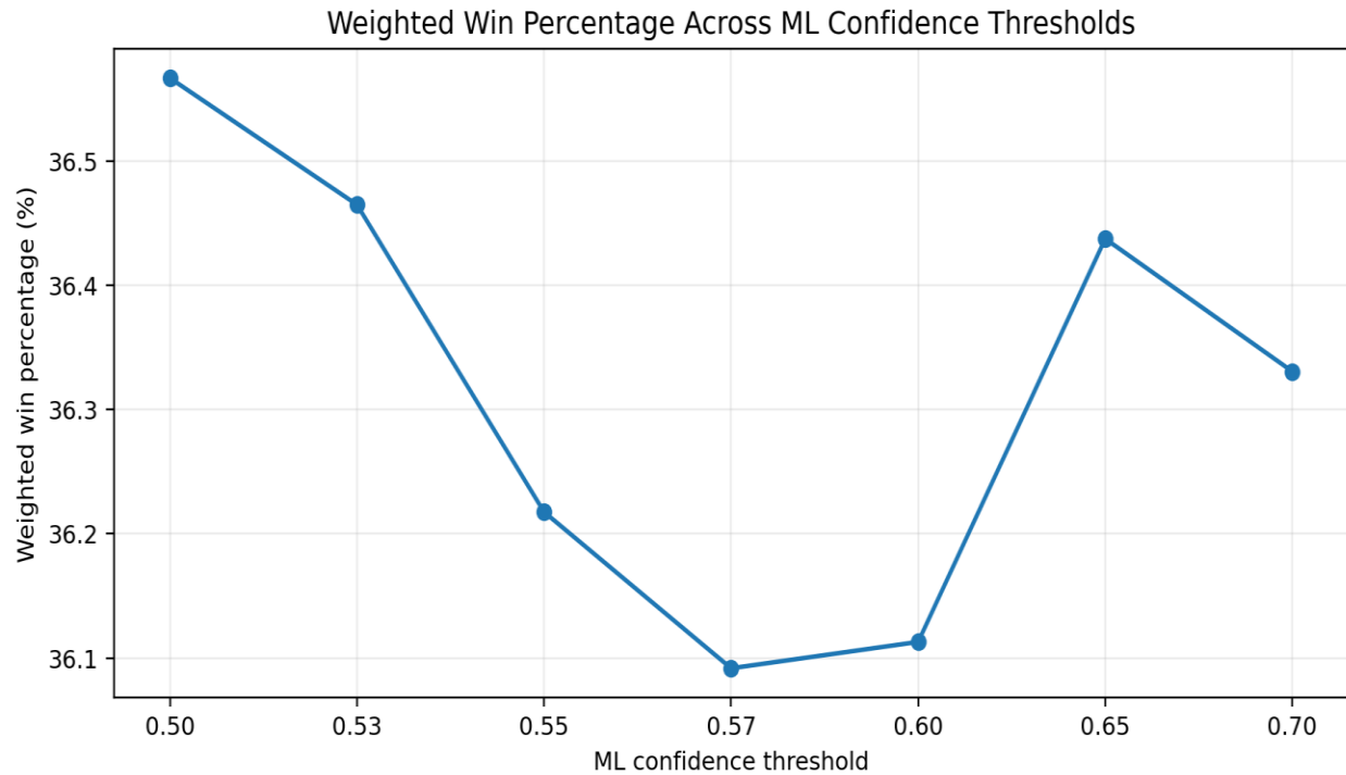
Figure 4. Weighted win percentage across the supplied ML-assisted experiment runs by confidence threshold.
