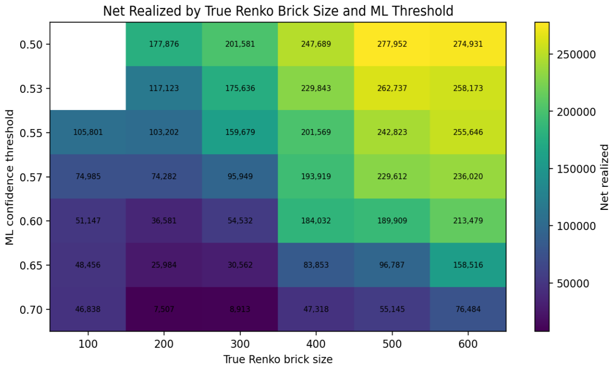
Figure 5. Net realized by True Renko brick size and ML confidence threshold.
