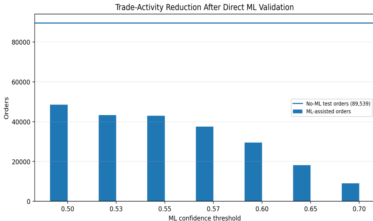
Figure 6. Reduction in trade activity after direct ML validation relative to the no-ML True Renko test reference.
