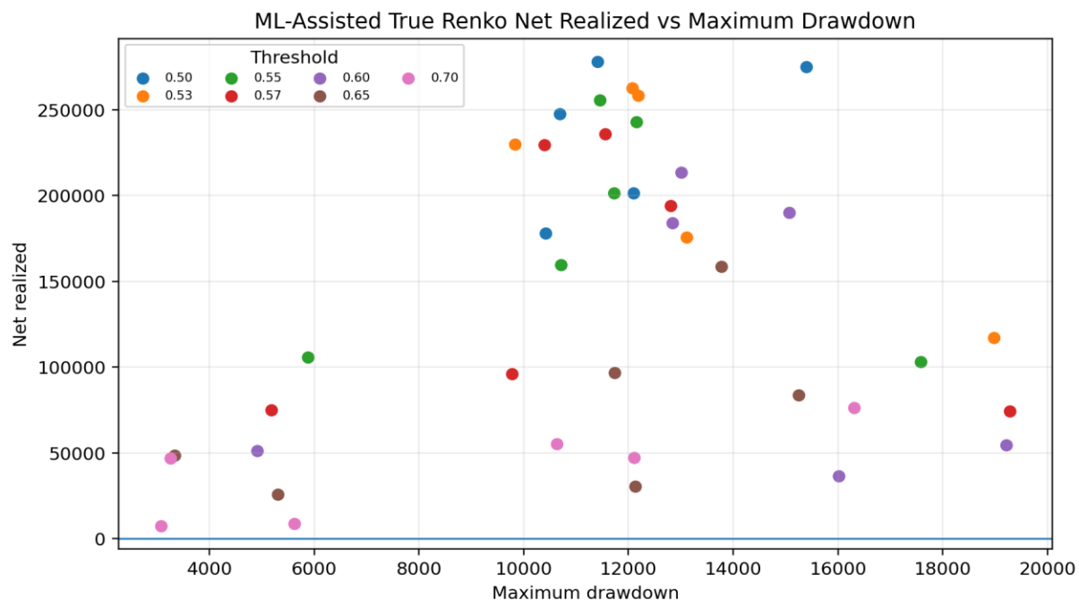
Figure 7. Net realized versus maximum drawdown for the supplied ML-assisted True Renko experiment runs.
