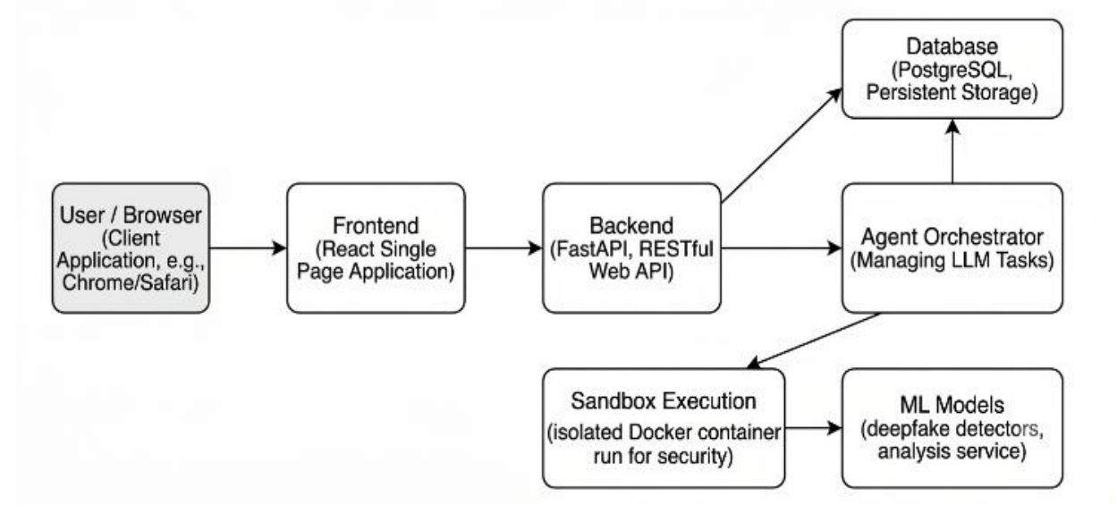
Fig. 1. System architecture of the AutoPatch AI framework
