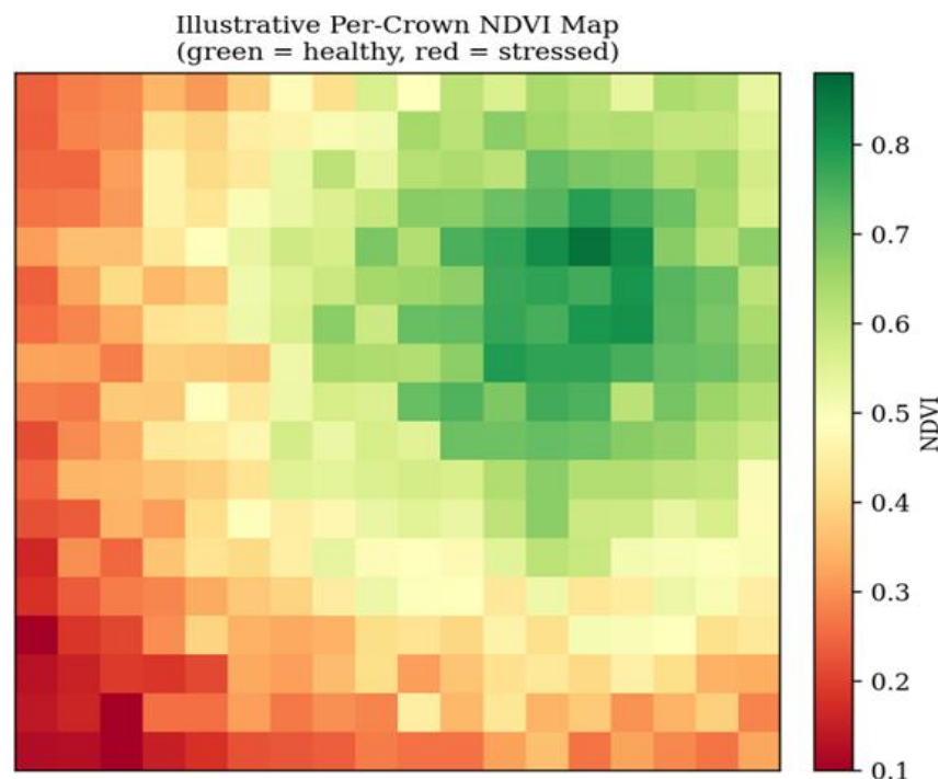
Figure 3. Illustrative per-crown NDVI map — greener cells indicate healthier canopy; red cells indicate stress.
