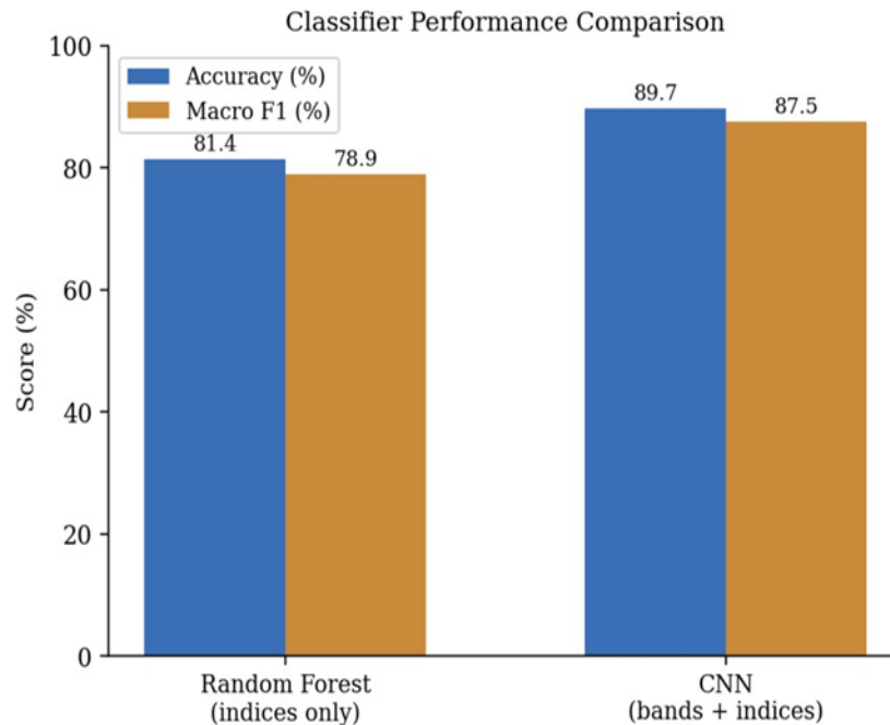
Figure 5. Accuracy and macro F1-score comparison between the Random Forest baseline and the CNN, corresponding to Table 2.
