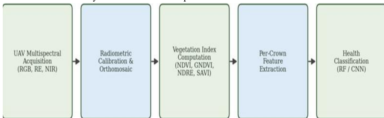
Figure 1. Proposed pipeline for multispectral tree health monitoring — acquisition, preprocessing, index computation, and classification.
