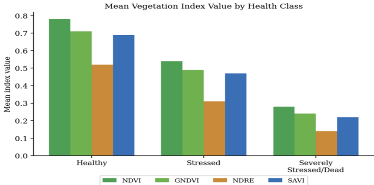
Figure 4. Mean vegetation index value by health class, corresponding to Table 1.
