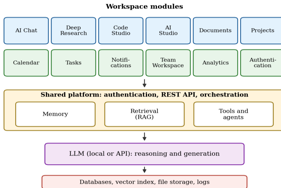
Fig. 1. Reference architecture of a modular AI workspace.
