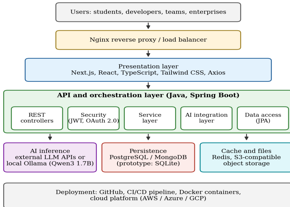
Fig. 2. ASTRA AI layered system architecture.
