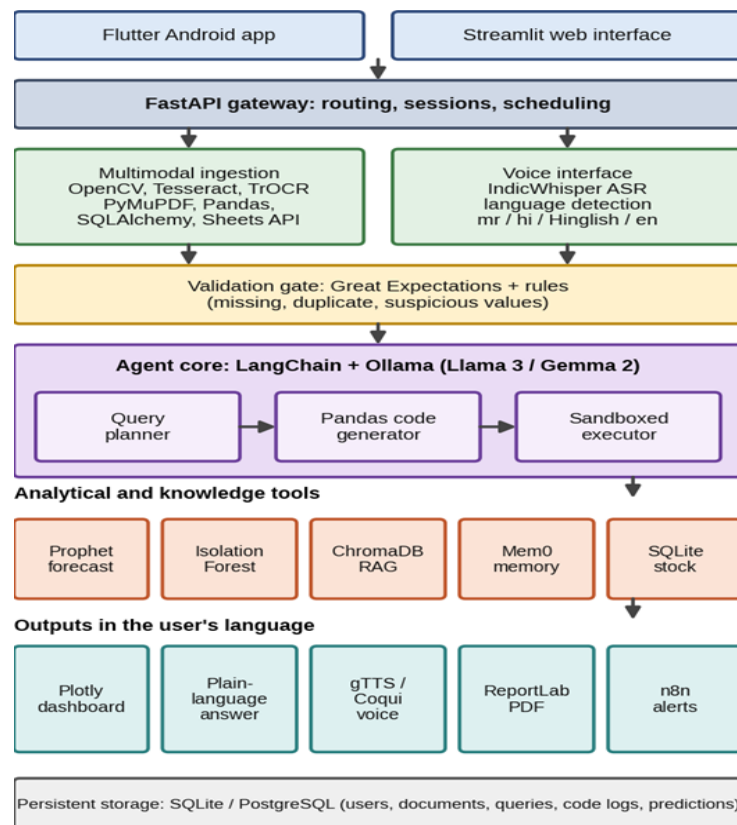
Fig. 1. Layered reference architecture of the proposed MMBIA system.
