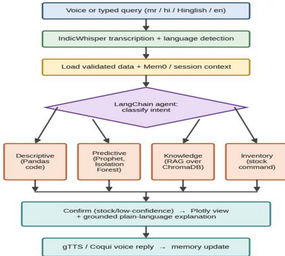
Fig. 2. Query routing workflow from voice input to spoken answer.
