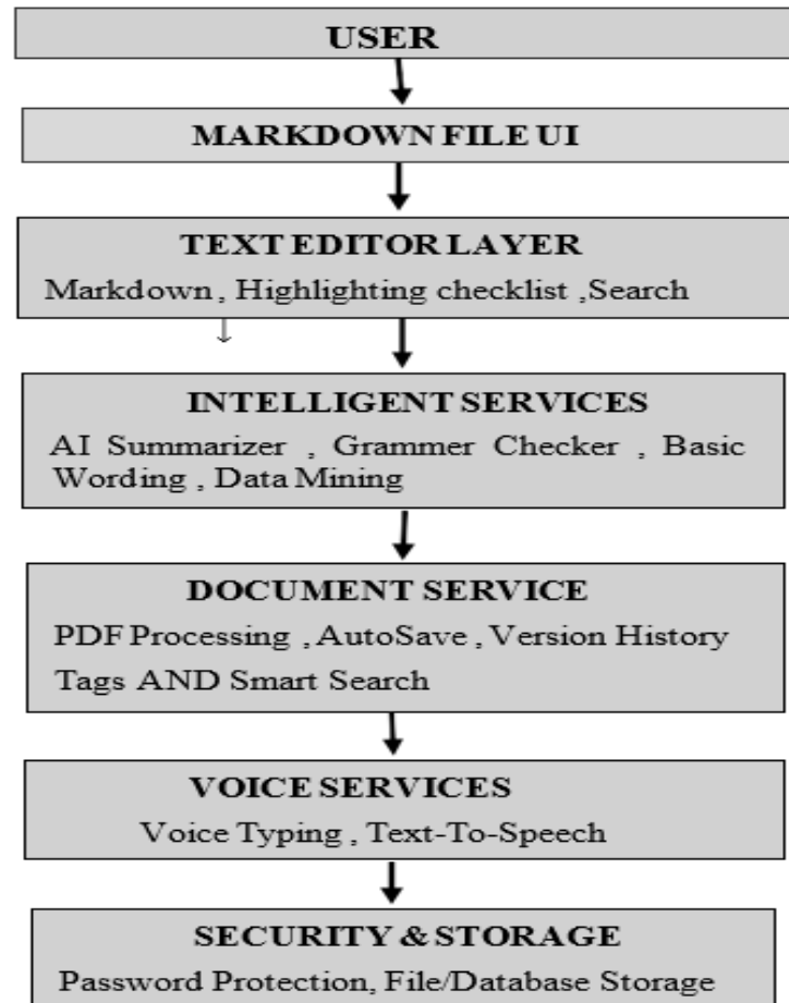
Fig. 1. Layered system architecture of Markdown File
