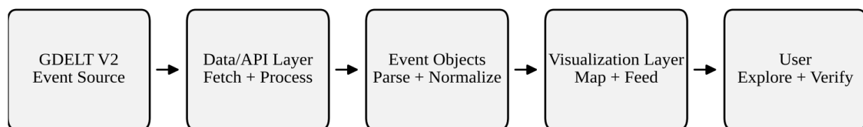
Fig. 1. Conceptual system architecture of WORLD CONFLICT MAP.
