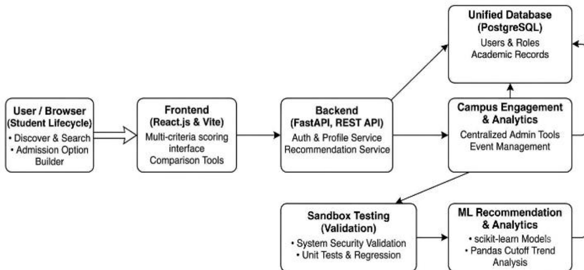
Fig. 1. System Architecture of the SMARTNEXUS Platform
