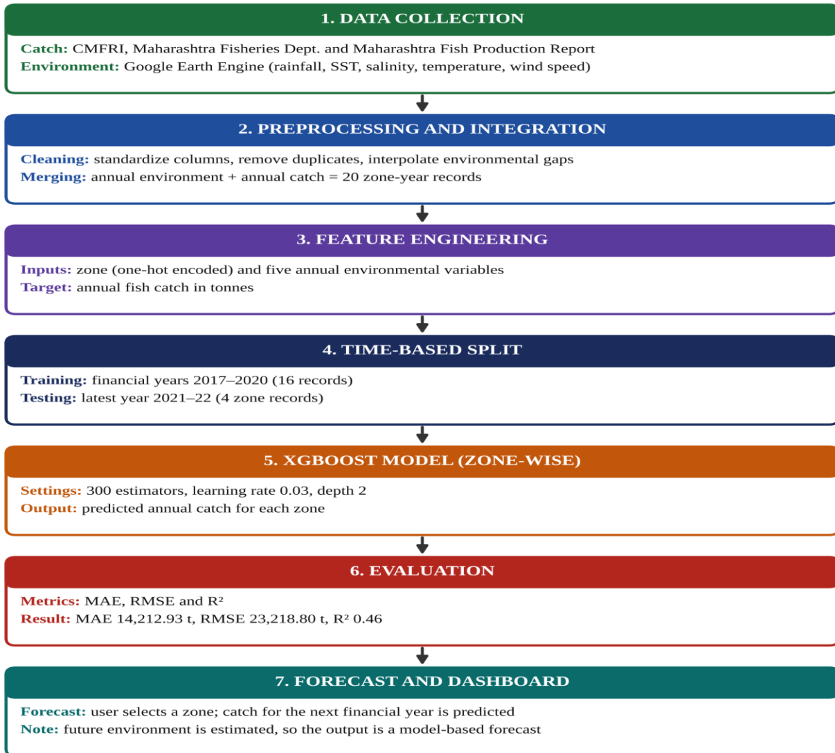
Fig. 2. Flow diagram of the zone-wise XGBoost fish catch prediction.
