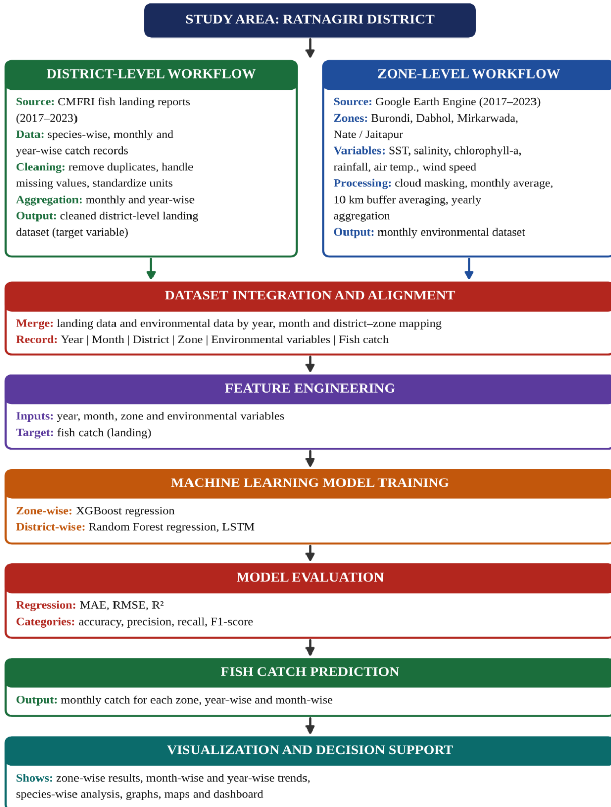
Fig. 1. System architecture of the machine learning AI based fish catch prediction system for Ratnagiri coastal fishermen using historical landing data.
