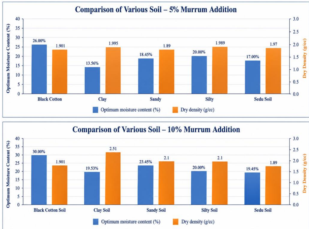
Fig. 1 and 2: Murrum added in various soil types in 5% and 10%
